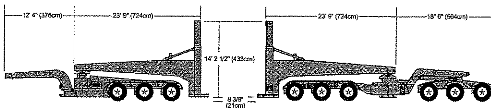
6 & 9 Axle Schnable with Steerable Dolly
